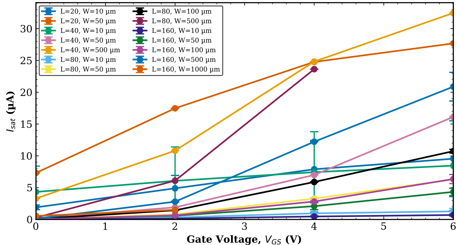
TFT2 Combined (Tr. 1 & 2) Saturation Current vs V_{GS} (mean \pm std)
